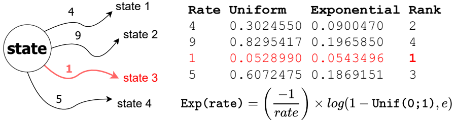
Figure 3.6: Drawing pseudo-numbers from uniform and exponential distributions to help simulate time in CTMC (log is the natural logarithm, in base e ).
